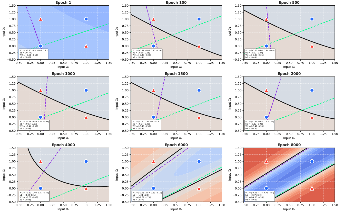
Figure 10: Evolution of the XOR decision boundary during neural network training. The colored regions represent the network's predictions, while the dashed lines show the decision boundaries formed by the hidden neurons at different training epochs.
